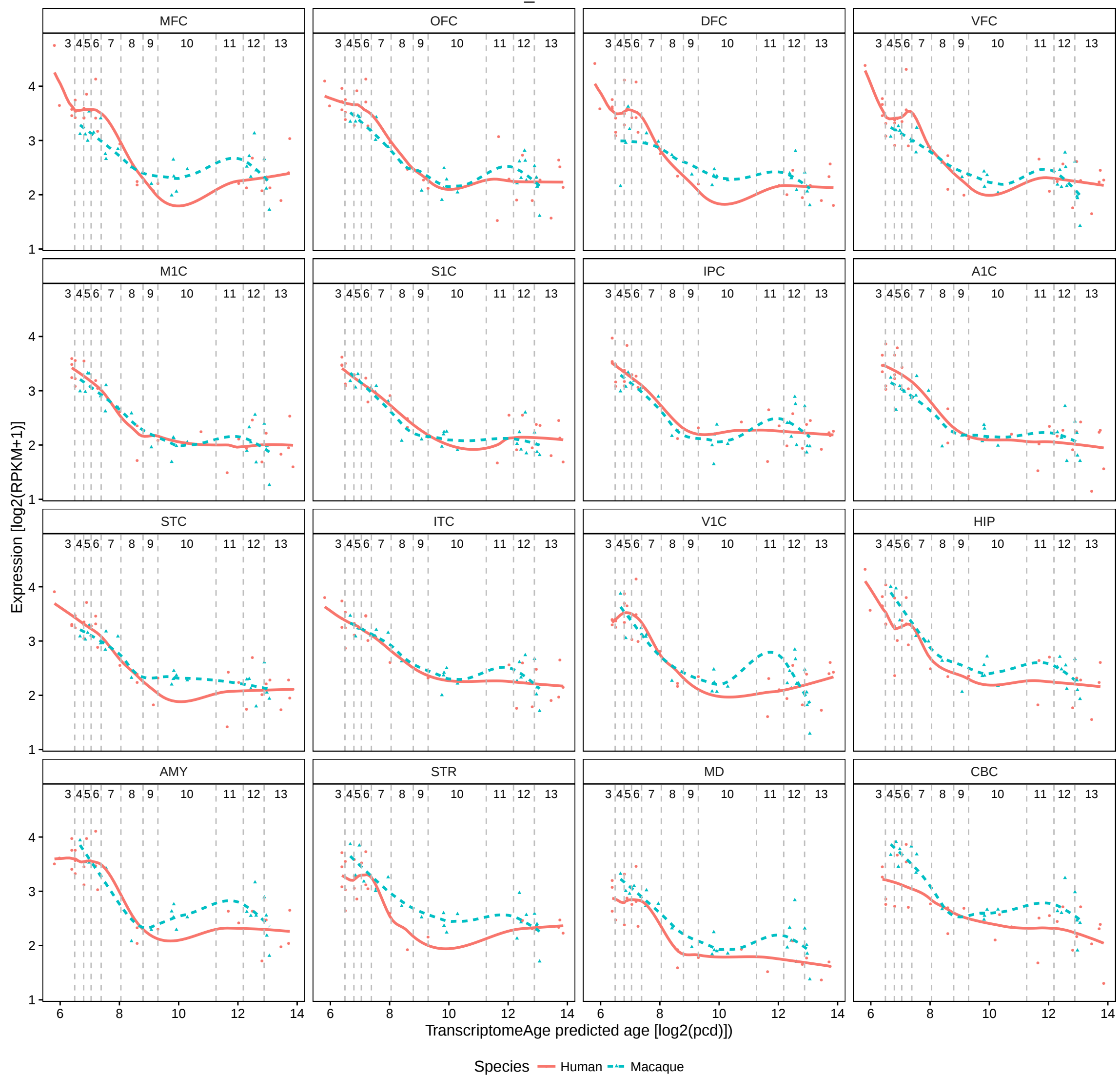
FIGNL1_ENSG00000132436
